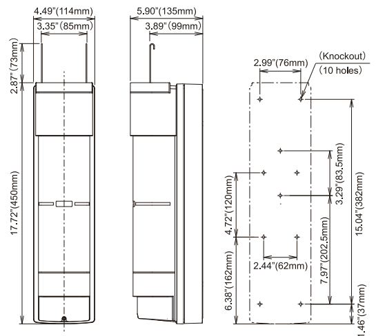
Reference installation drawing
